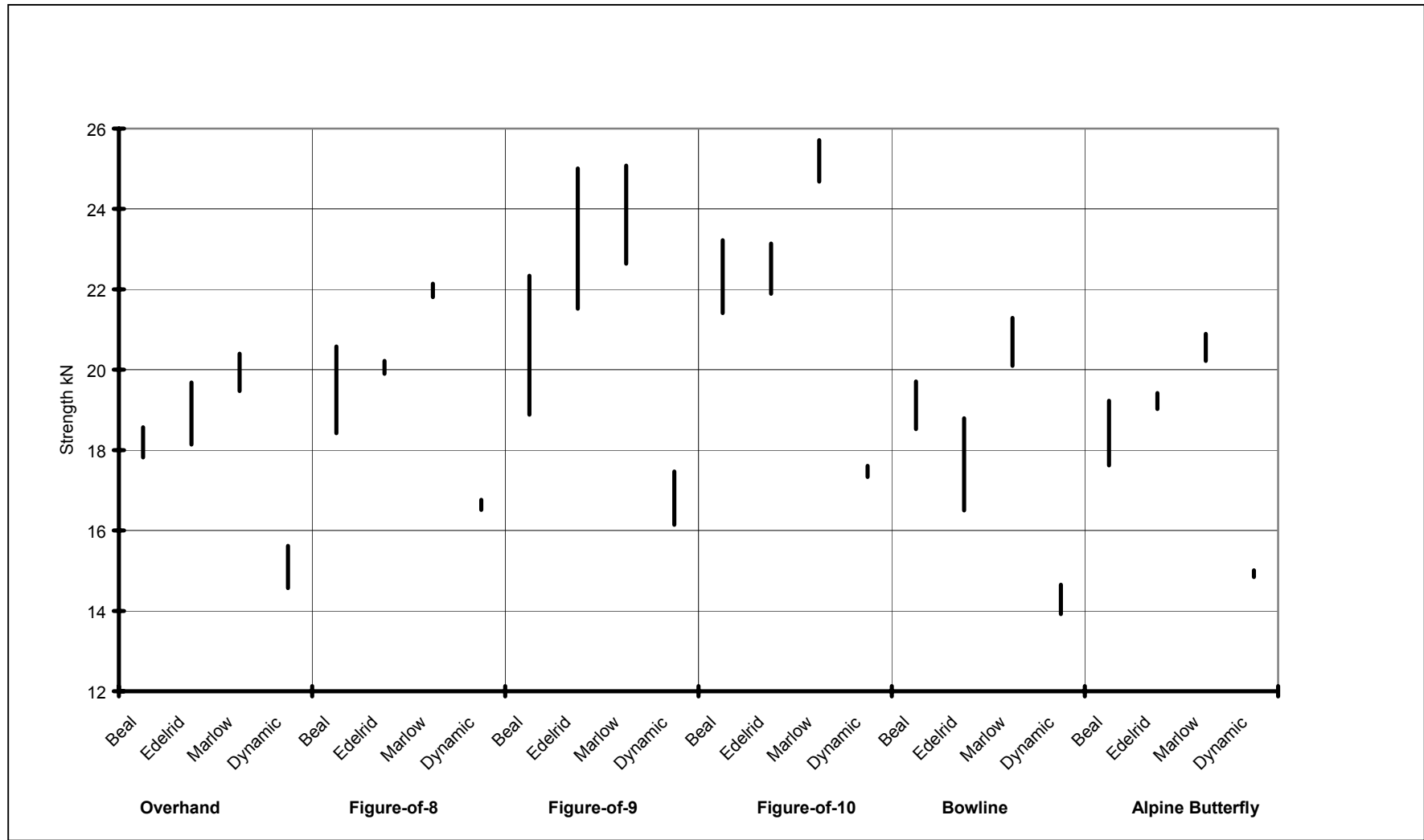
Figure 13 Knot strength (absolute)
