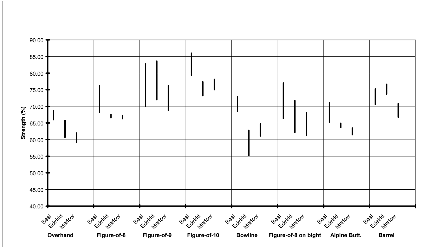
Figure 12 Knot strengths (percent of manufacturers' stated strength)
